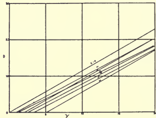
D- \gamma Curves for KBr concentrations 0, .01, .02, .04, .08, .16 and .32 M.
